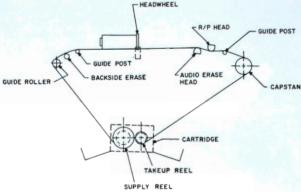
FIG. 5 Automatic tape threading path.
