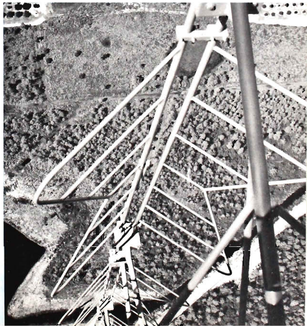
FIG. 5 (lower left) Another view from service elevator, inside tower, showing part of antenna feed system and junction box.
