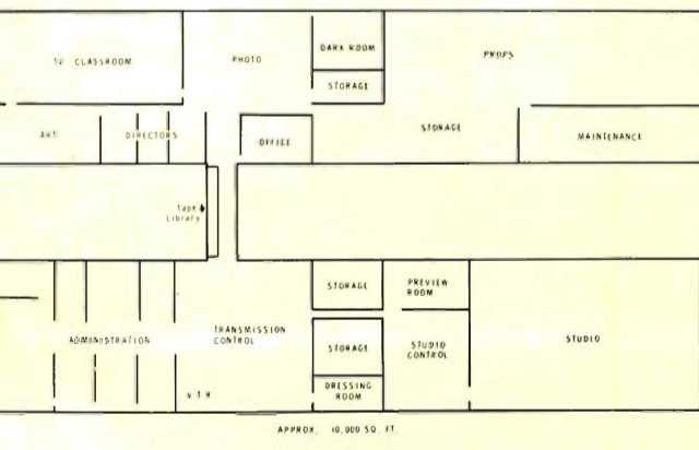
FIG. 8 All major facilities are centrally located for smooth production and distribution.
