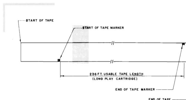
FIG. 3 Locations of mechanical cue markers.
