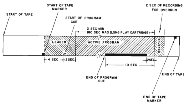
FIG. 4 Format of the recorded cartridge tape.
