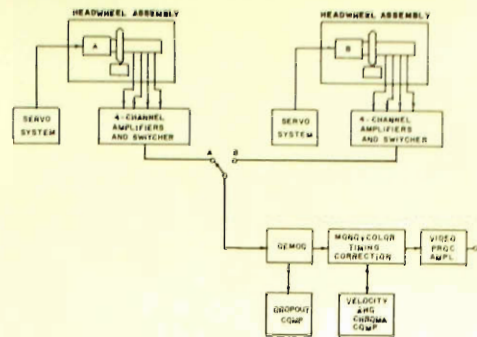
FIG. 10 Electronic system block diagram for cartridge playback.
