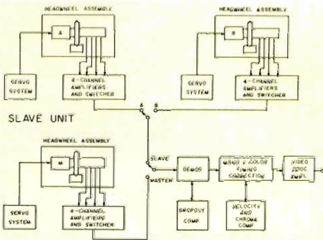
FIG. 11 Block diagram slave/master machine electronics.
