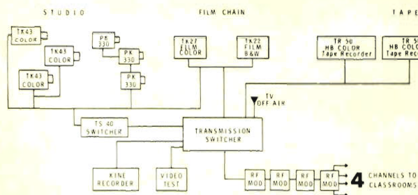
FIG. 7 Simplified schematic of originating, switching, and transmission equipment.
