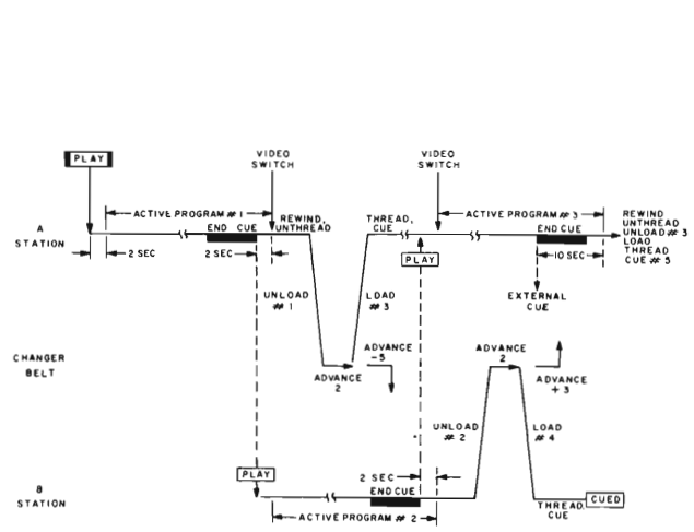
FIG. 8 Three-cartridge operations sequence.
