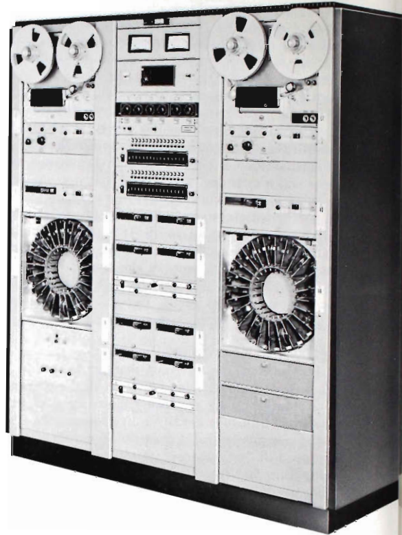
"Building block" units of RCA Automation systems
